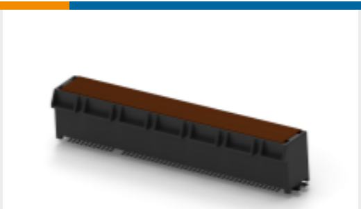
TE Part #5-2337939-7 PCIE GEN4 CON,SMT,98POS,30u\", MYLAR,HT
