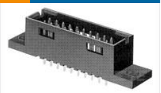
TE Part #87474-2 20 MODII HDR DRST SHRD .100CL
