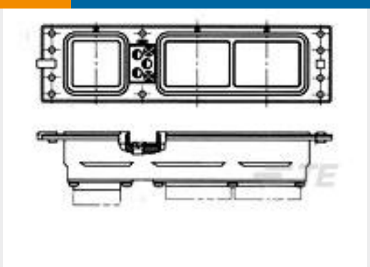
TE Part #208970-6 CONNECTOR, SIZE 2 RECEPT-NIC60
