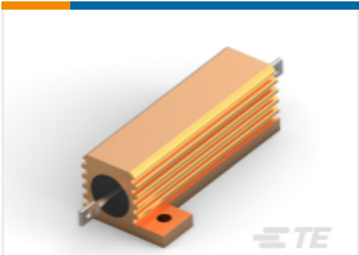
TE Part #1676814-7 Power Resistors: Aluminum Housed, HSA
