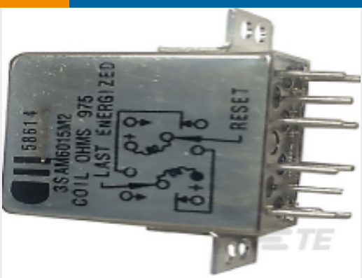
TE Part # 8-1617349-9 3SAM1821A2=M39016/32-003
