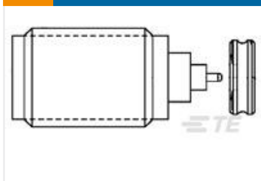
TE Part #1053254-1 2058 5278 00 SMA FEEDTHRU JACK, SEALED
