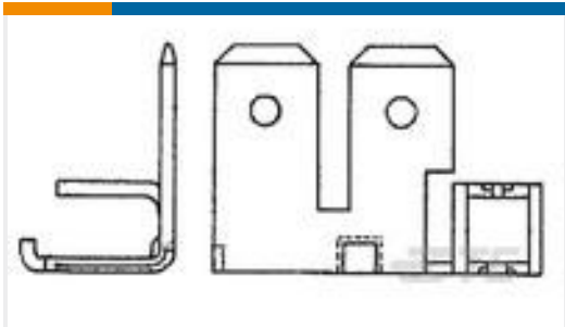
TE Part #444070-2 TERMINAL BOARD INS DISPLAC 6.3 TAB BR
