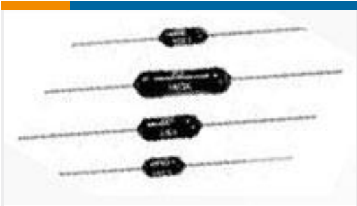
TE Part #1-1879682-1 H8 12R7 0.1% 50PPM
