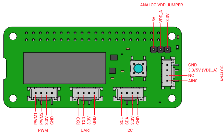
Figure 2. Pin functions for each Grove connector
