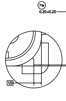
VIEW AF KEY TYPE 1
