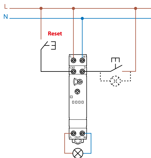
Type 13.61.8.230 - Examples of multiple 4 wire connection with centralized reset push-button
