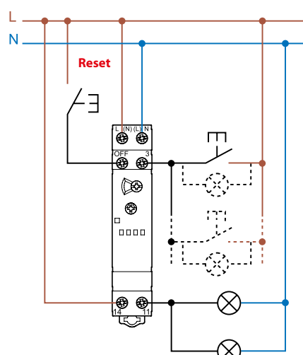
Type 13.62.8.230 4 wire connection
