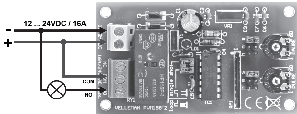
CONNECTION EXAMPLE: LOW VOLTAGE (12 ... 24VDC)
