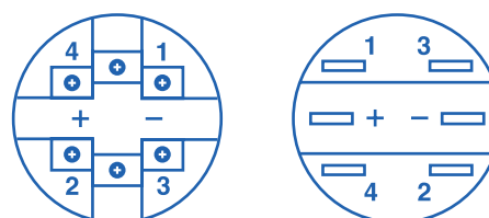
Screw Layout
