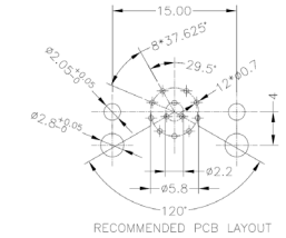
12 Contact PCB Layout
