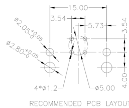
5 Contact PCB Layout
