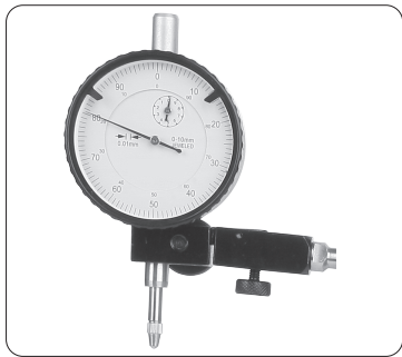
holding stem \Phi 8\text{mm} in metric/ 3/8'' DIA in inch
