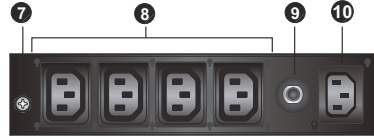
PE4104AJ (Rear)
