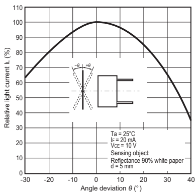
Fig 10. Sensing Angle Characteristics (Typical)
