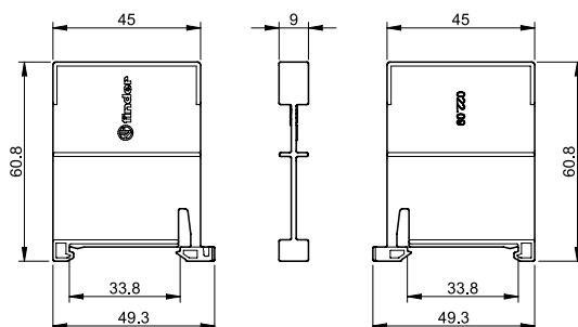
Separator for rail mounting, plastic, 9 mm wide
