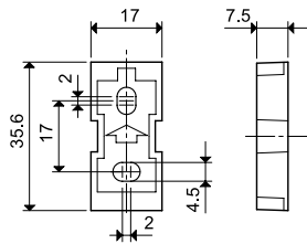
Adaptor for panel mounting, plastic, 17.5 mm wide for 70.11 and 70.61
