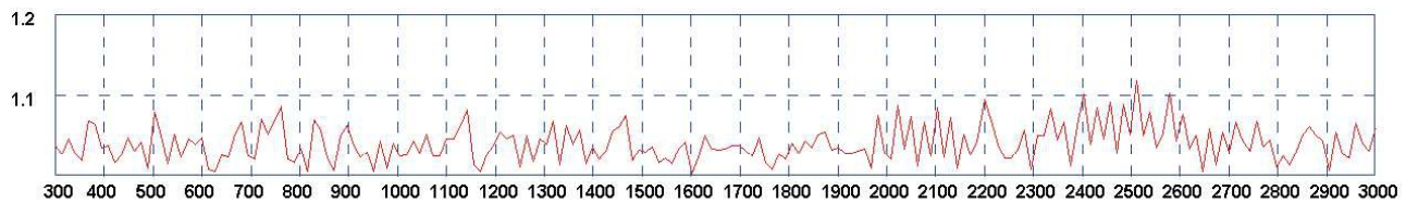
Typical VSWR*
