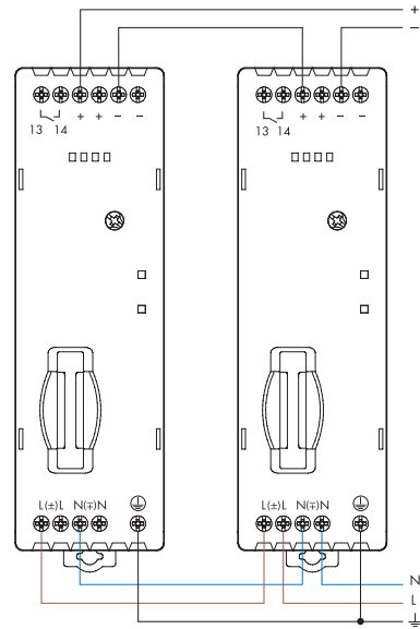
Series connection
