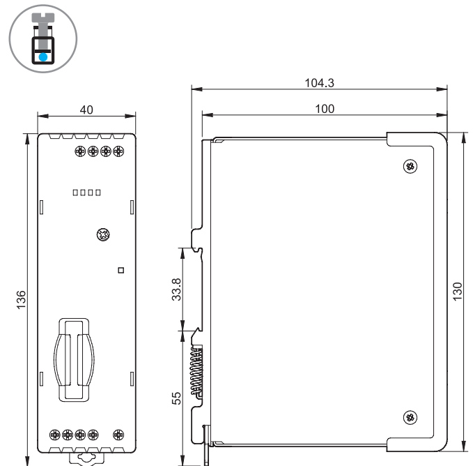
78.1B Screw terminal
