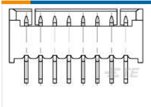
TE Part #1734598-5 1.25 WTB HDR DIP, 5 POS
