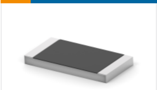
TE Part #1622820-8 SMD Power Resistor: 1 Watt, 3520 Series
