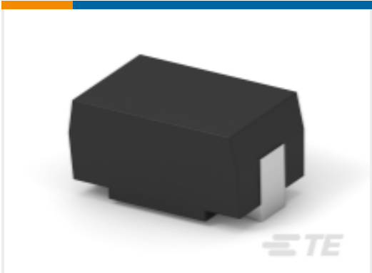
TE Part #1-1879022-3 SMD Power Resistor: 7 Watt, 200-2M Ohm
