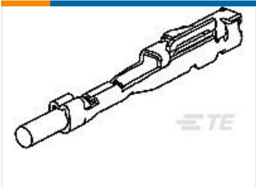
TE Part #1123343-2 025 REC CONTACT GOLD FORMING
