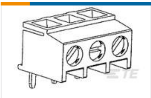
TE Part #284093-4 TERMI-BLOK PCB MOUNT 90, 5,0MM
