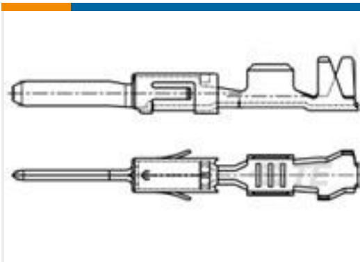
TE Part #963904-2 TAB A 1.6x0.6 CONTACT CF SWS Sn
