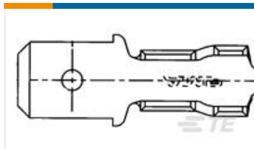
TE Part #41411 250 FASTON,TAB,18-14 AWG,BR
