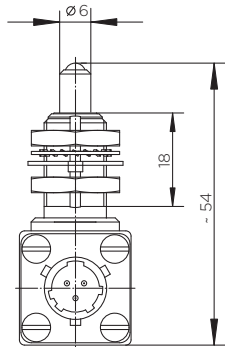
Example G13-01-1167 (SILVER)
