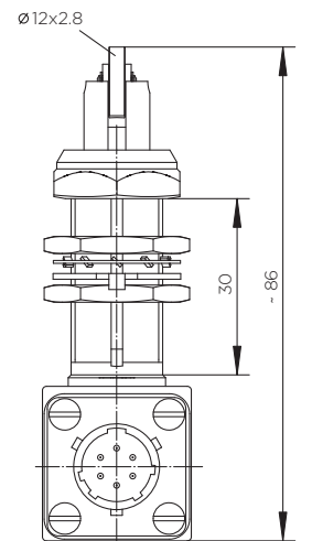
Example G13-01-1365 (2-POLE, SILVER)
