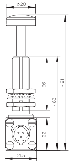
Example G13-01-1133 (SILVER)
