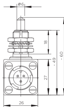
Example G13-01-1097 (1-POLE, SILVER)
