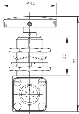
Example G13-01-1220 (2-POLE, SILVER, RED) G13-01-1629 (2-POLE, GOLD, RED) G13-01-1585 (2-POLE, SILVER, GREEN) G13-01-1470 (WITH CONNECTOR CECC 7520, RESISTANT TO SALTWATER)
