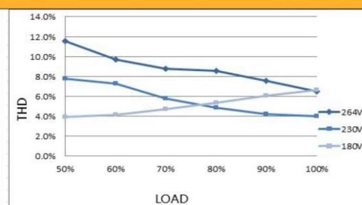
Fig.5 Total harmonic distortion curve (THD)
