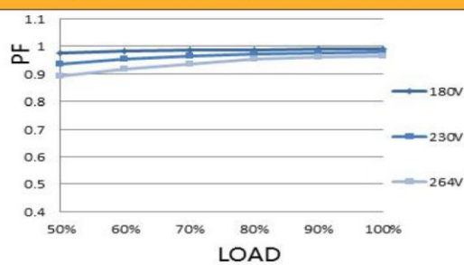
Fig. 4 Power factor characteristic curve
