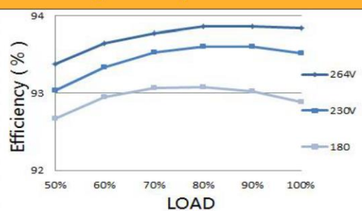
Fig.6 Efficiency-Load curve
