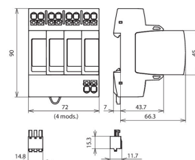
Dimension drawing DG MP TNS 275 FM
