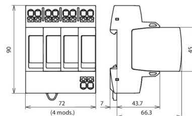
Dimension drawing DG MP TNS 275
