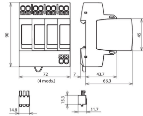
Dimension drawing DG MP TT 275 FM
