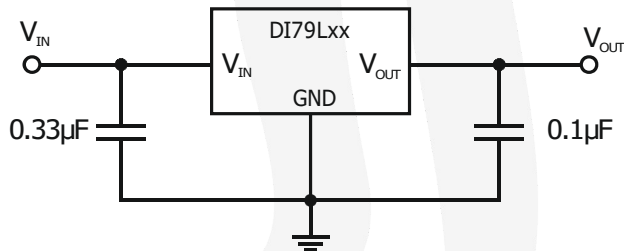
Fig. 1 Typical application circuit for DI79LxxDAB
