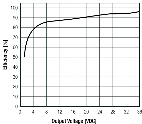
Efficiency vs. Output Voltage
