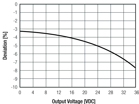
Deviation vs. Output Voltage
