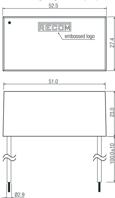
Dimension Drawing Single Wired (mm)
