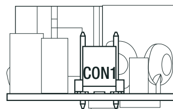
AC Input Side View
