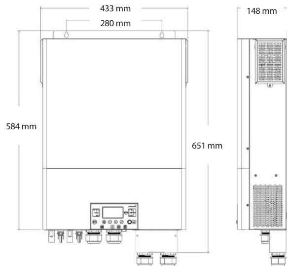
PSW-H-5KW-120/48V, PSW-H-6.5KW-120/48V and PSW-H-8KW-230/48V* *only the PSW-H-6.5KW-120/48V model includes bottom greyed out extension box
