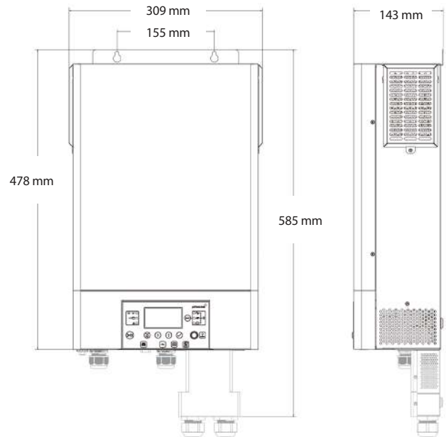
230 Vac models and PSW-H-3KW-120/24V* *only the PSW-H-3KW-120/24V model includes greyed out bottom cable glands and extension box
