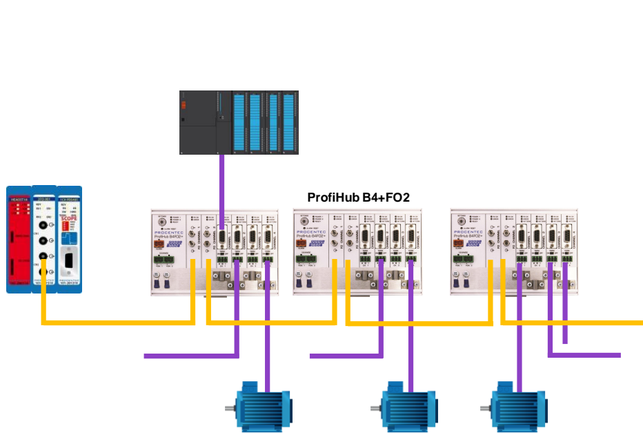
Fig. 4 - Creating a fiber optic backbone increases network reliability and network overview. It is also possible to mix ProfiHubs with ComBricks
