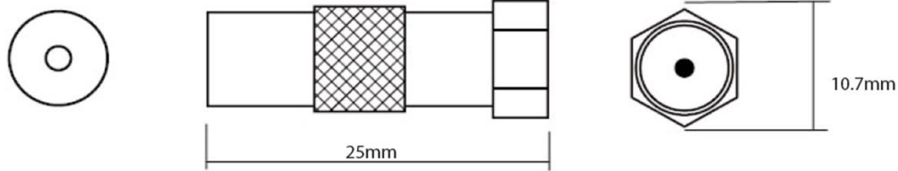
IEC-Buchse / F-Stecker IEC-jack / F-plug
