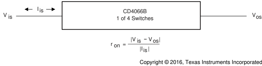
Figure 6-1. Determination of r_{on} as a Test Condition for Control-Input High-Voltage ( V_{IHC} ) Specification
