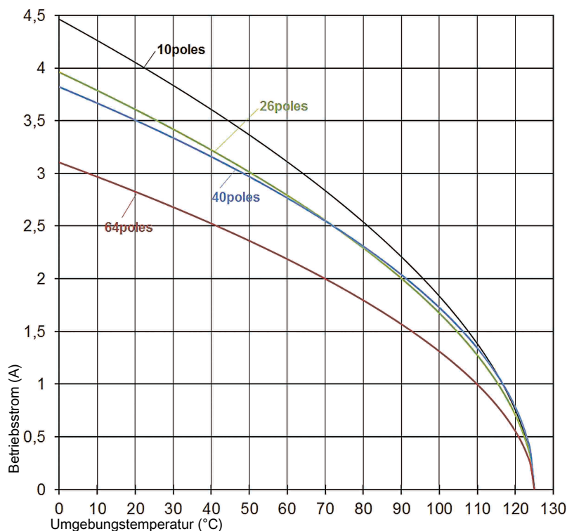
Deratingkurve 80%
