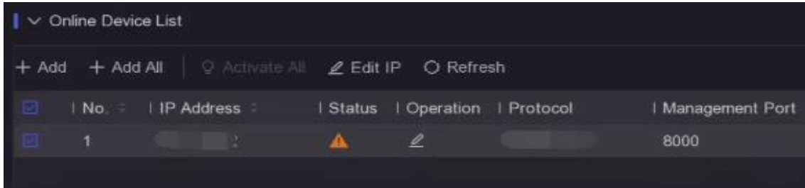
Figure 6-8 Online Device
