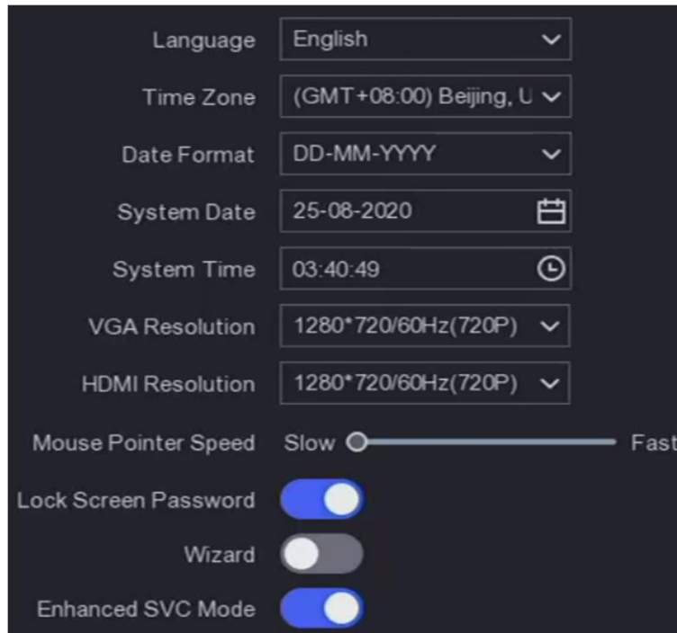
Figure 6-1 Basic Settings
