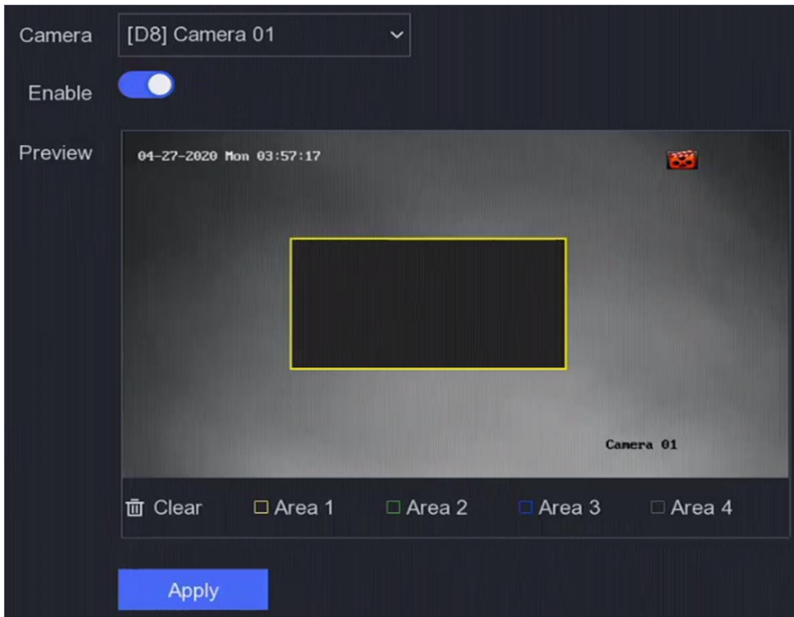
Figure 6-13 Privacy Mask
