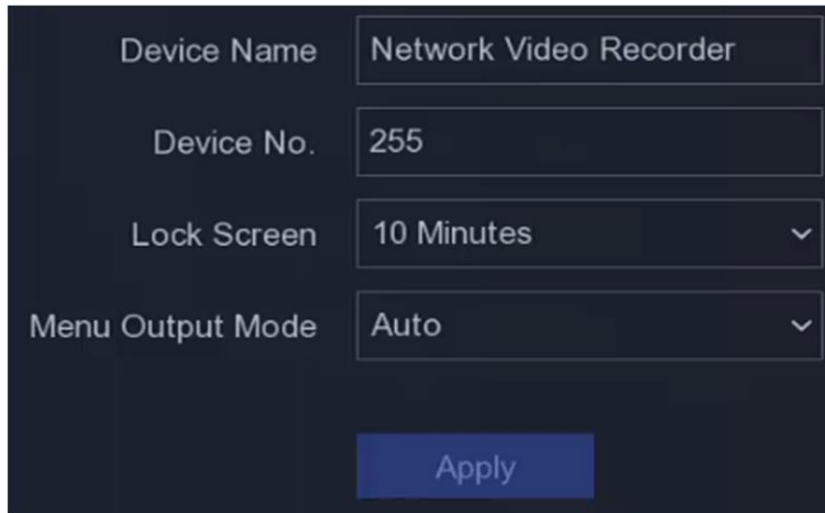
Figure 6-2 More Settings
