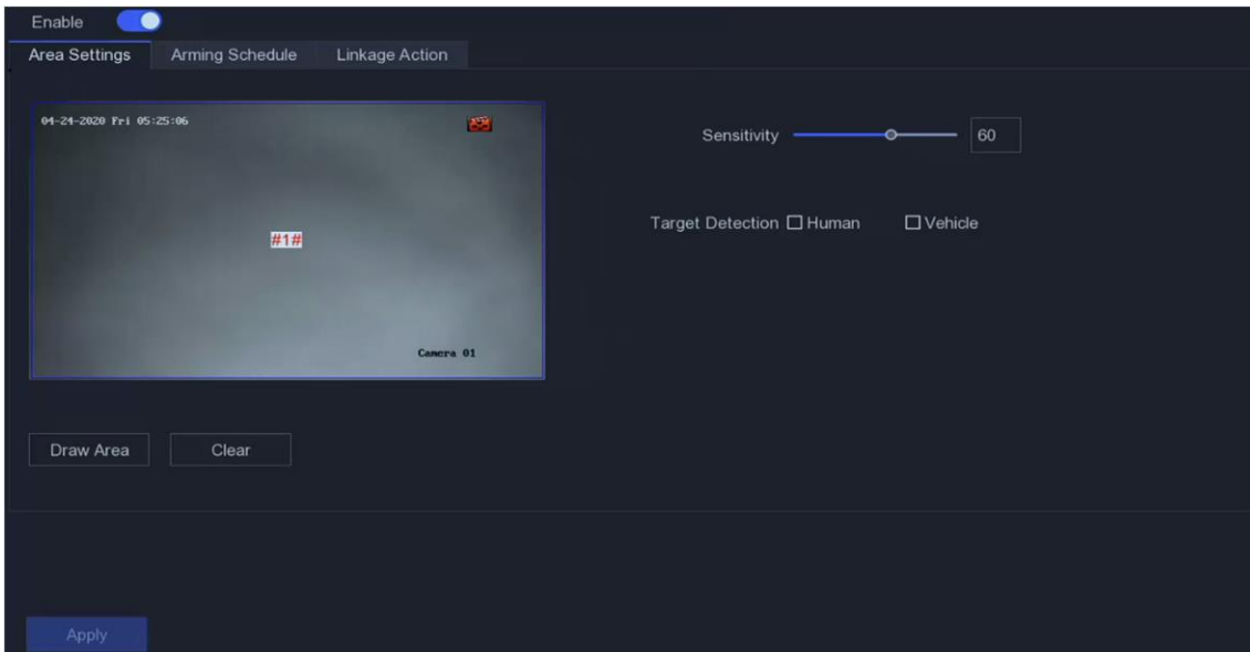
Figure 5-10 Motion Detection
