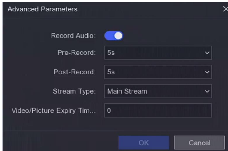
Figure 6-23 Advanced Parameters
