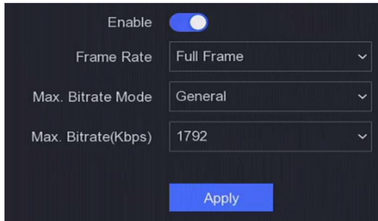
Figure 6-4 Channel-Zero
