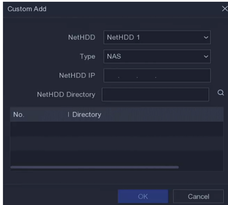
Figure 6-24 Add NetHDD
