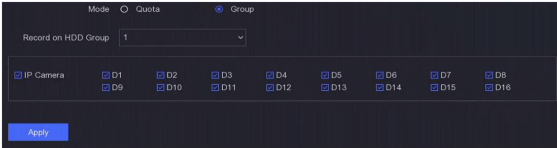
Figure 6-25 Group
