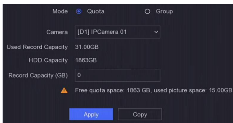
Figure 6-26 Quota
