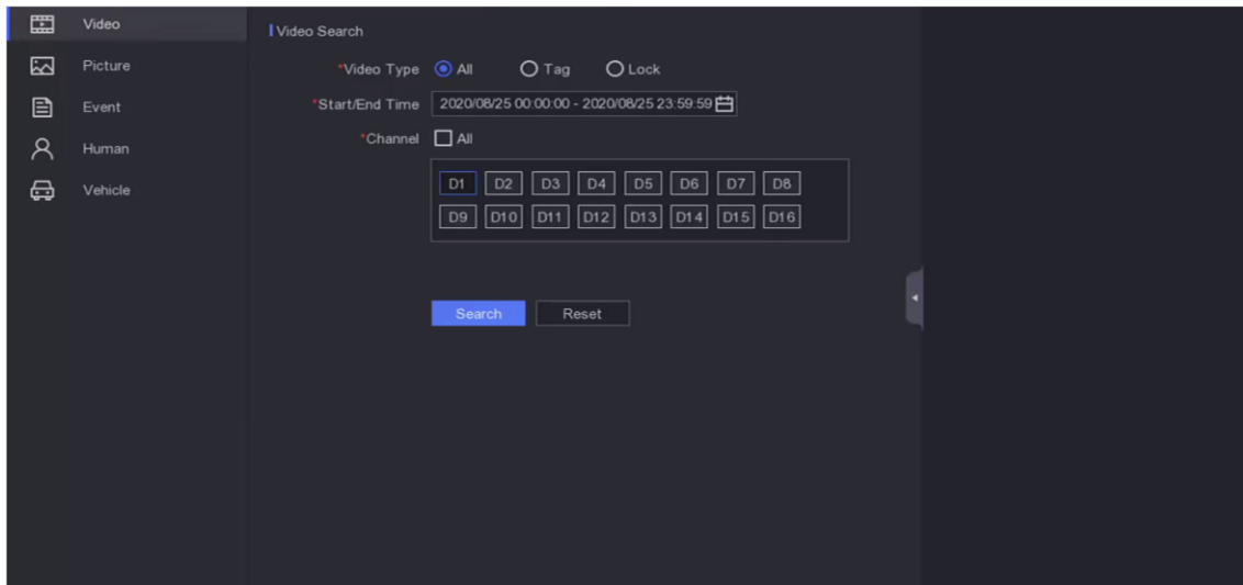
Figure 4-1 Search
