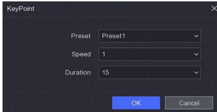
Figure 2-3 Patrol Settings
