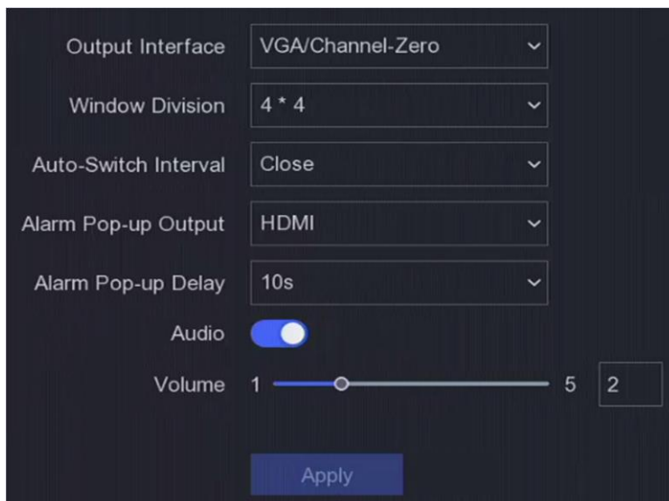
Figure 6-3 Live View-General
