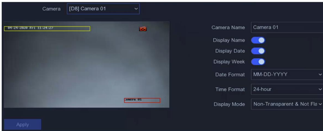
Figure 5-9 OSD
