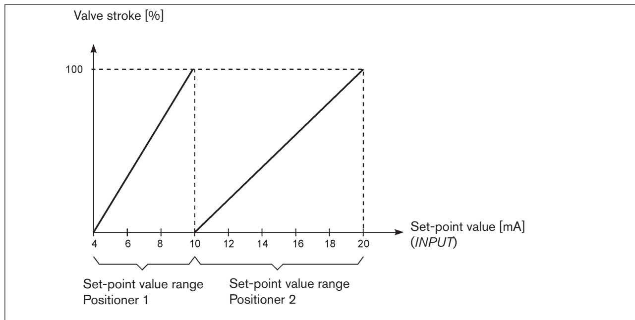
Fig. 37: SPLTRNG graph
