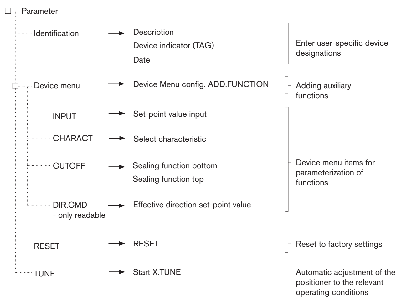
Fig. 18: Navigation area
