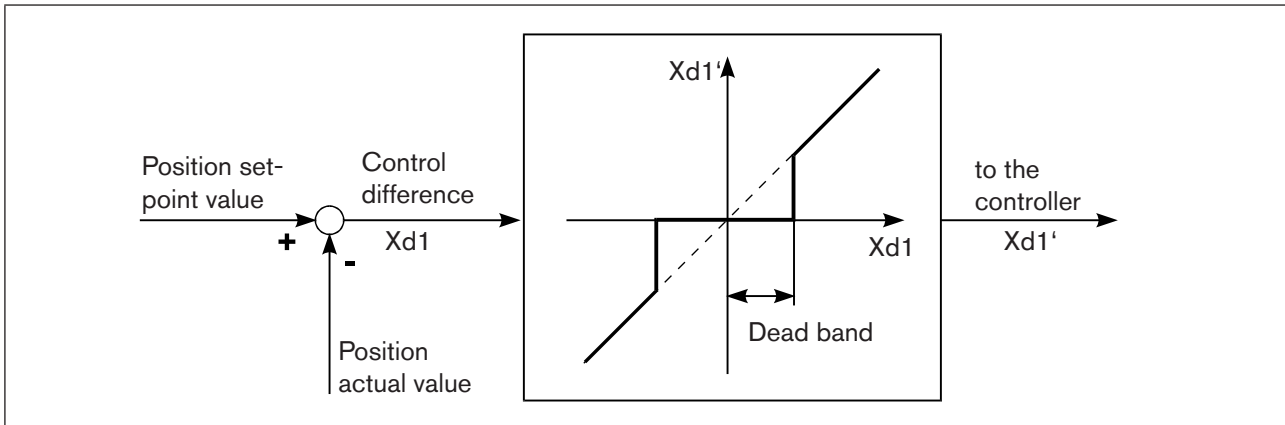
Fig. 43: X.CONTROL graph
