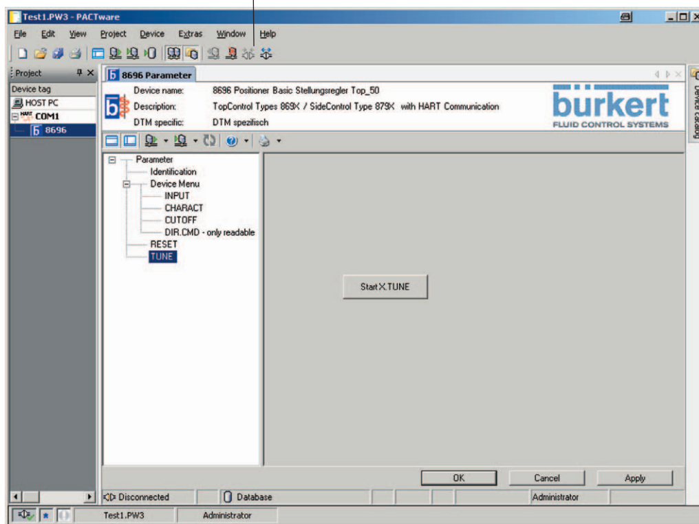
Fig. 20: Starting X.TUNE
