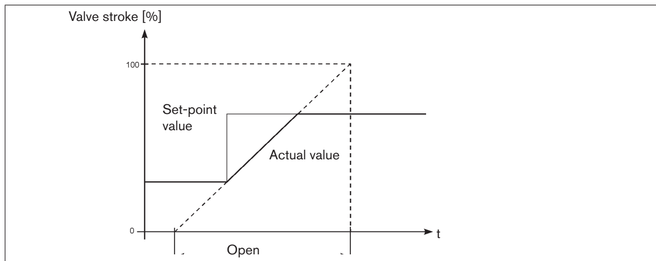
Fig. 41: X.TIME graph
