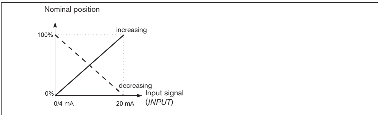
Fig. 31: DIR.CMD graph
