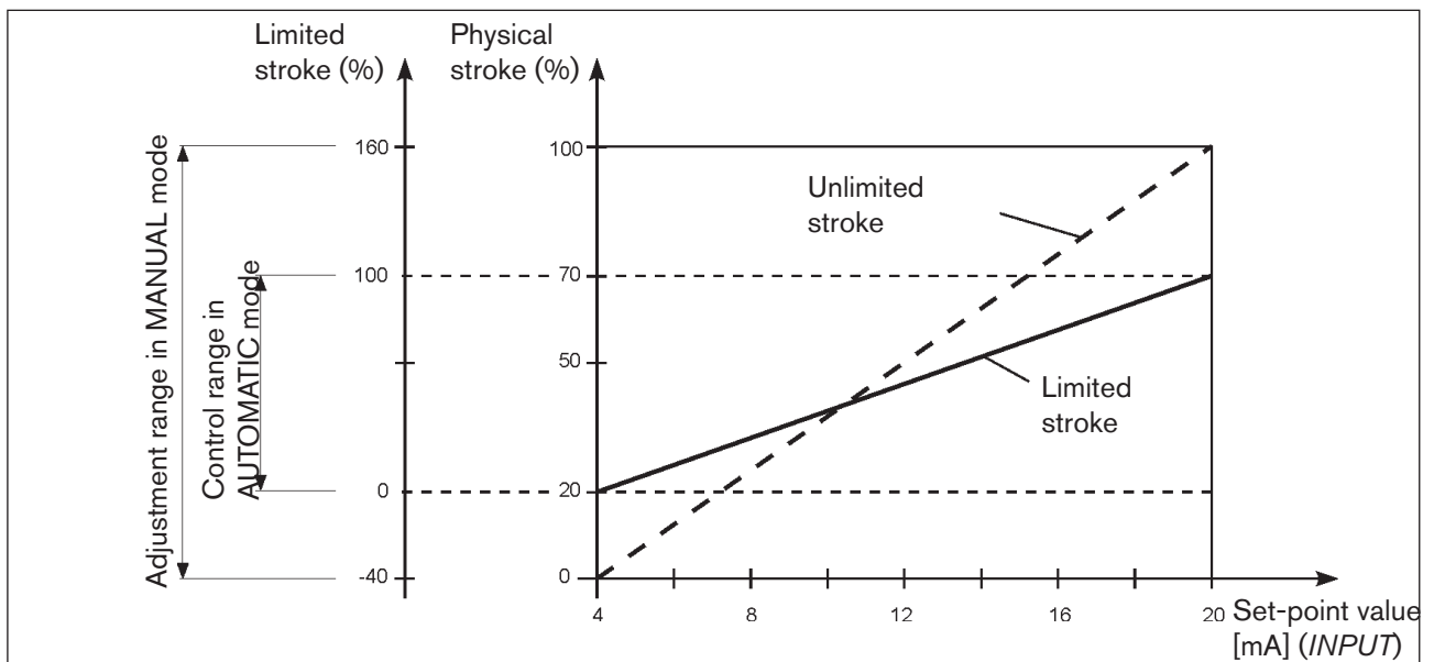
Fig. 39: X.LIMIT graph
