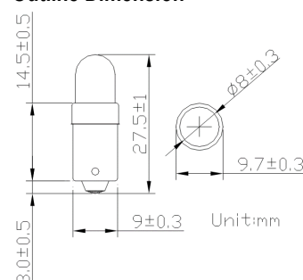
Outline Dimension
