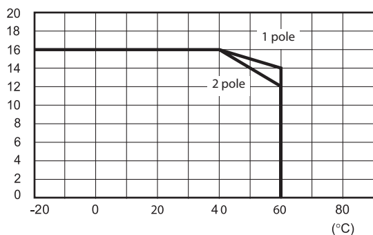
L 12 - Rated current v ambient temperature
