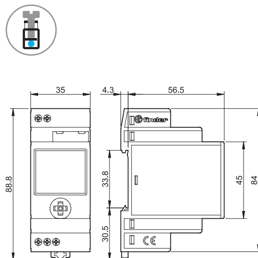
Types 12.61 / 12.A1 Screw terminal
