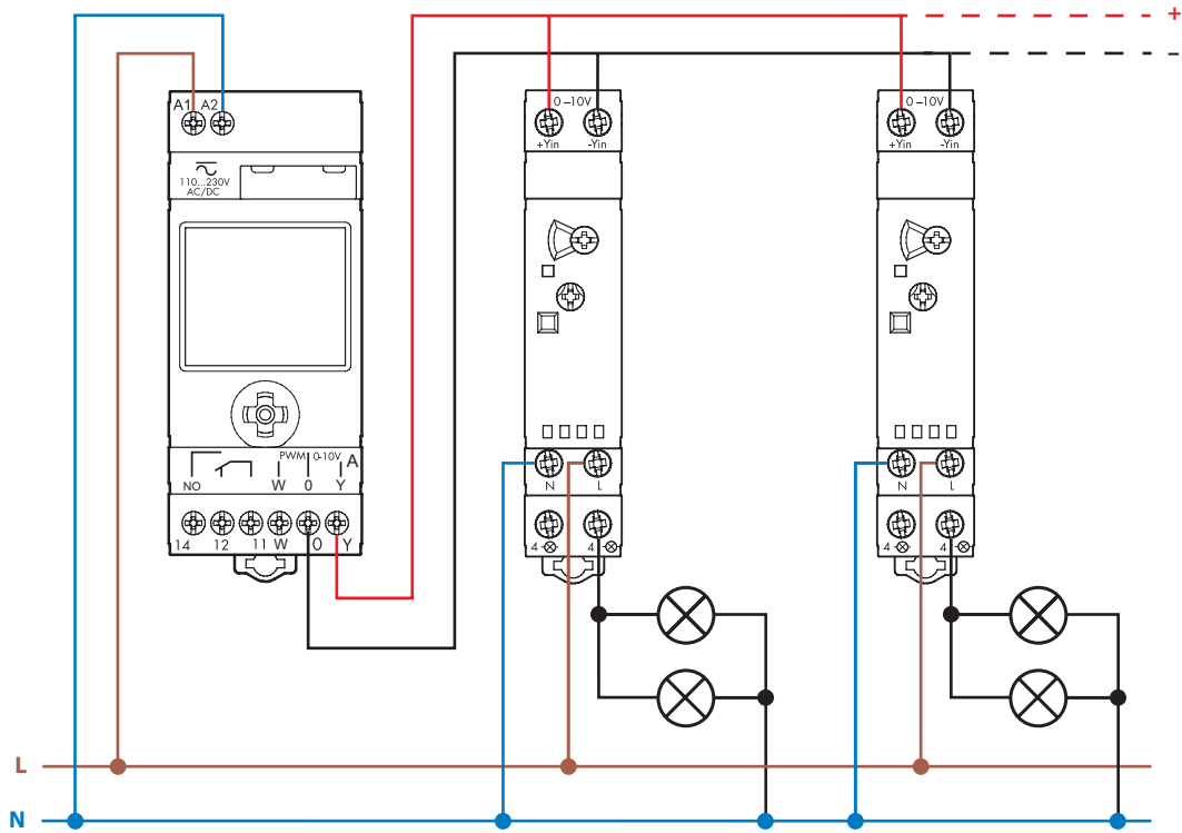
Type 12.A4 with 15.11 Application example with slave dimmer Type 15.11
