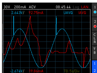
Trend chart function
