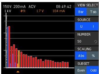
Harmonic analysis function
