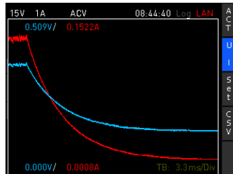
Inrush function
