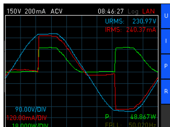
Waveform function
