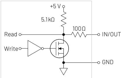
I/O 1–9
