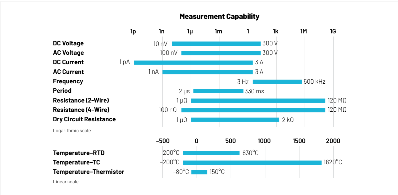
Measurement capabilities of the high performance multimeter
