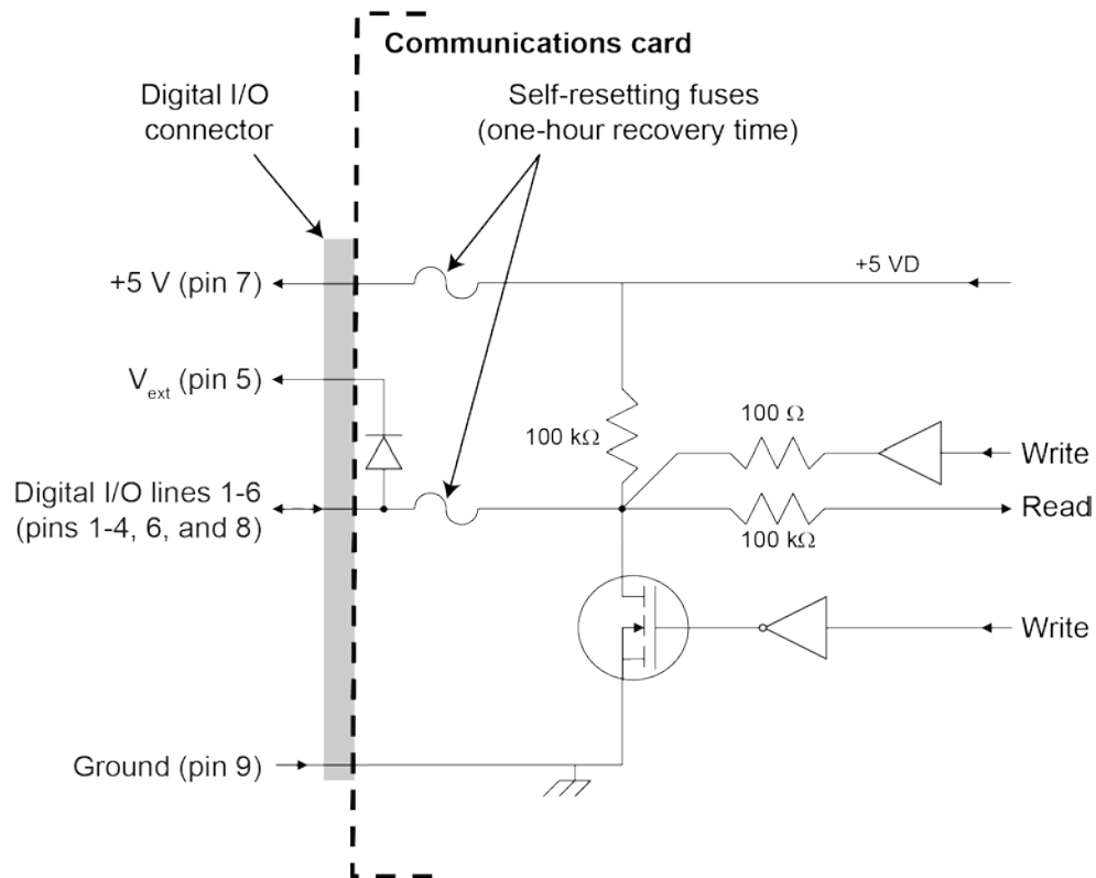
Figure 5: Digital I/O port configuration
