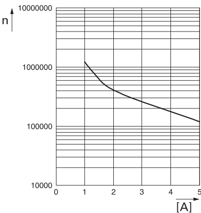
Figure 11: Number of switching cycles DC-13
