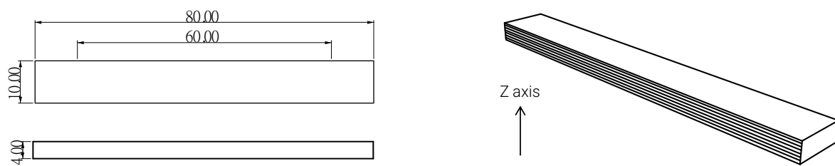
Fig 2. Flexural testing specimen
