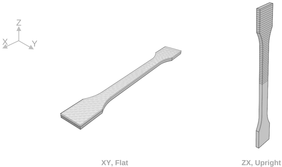
Fig 4. Print Orientation
