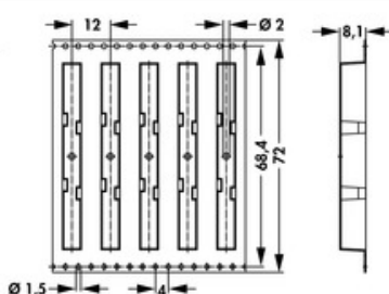
MK 23 SMD ... 14-20 B TR
